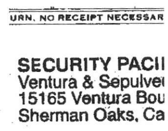
Figure 8. Binary image.
