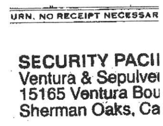
Figure 8. Binary image.
